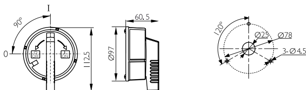
DVACC8003/4DB. SWITCH HANDLE (BLACK) (Ø97mm)
