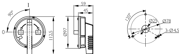
DVACC8003/IDB. SWITCH HANDLE (BLACK) (Ø97mm)
