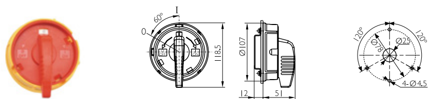
DVACC8003/3DE-I. INTERLOCKING ELEMENT FOR SAFETY EMERGENCY STOP SWITCH HANDLE (RED / YELLOW) (Ø107mm)
