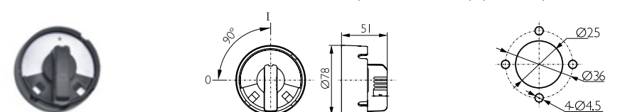
DVACC8003/5TD. OPERATION HANDLE (GREY / BLACK) (Ø78mm)
