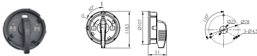
DVACC8003/3DB. SWITCH HANDLE (BLACK) (Ø107mm)
