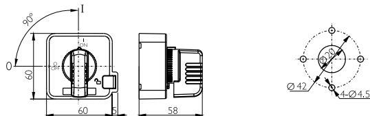
DVACC8029/IBB. SWITCH HANDLE (GREY / BLACK) (60x60mm)
