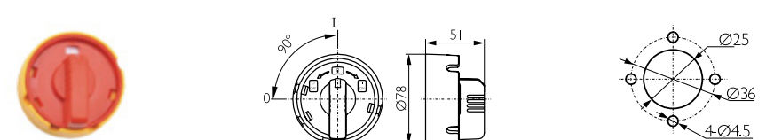
DVACC8003/5PE. EMERGENCY OPERATION HANDLE (RED / YELLOW) (Ø78mm)
