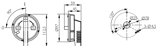
DVACC8003/IDE. EMERGENCY SWITCH HANDLE (RED / YELLOW) (Ø97mm)
