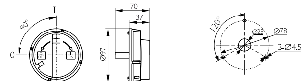
DVACC8003/2DA. MOTOR SWITCH HANDLE (GREY / BLACK) (Ø97mm)
