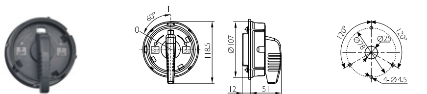
DVACC8003/3DB-I. INTERLOCKING ELEMENT FOR SAFETY SWITCH HANDLE (BLACK) (Ø107mm)
