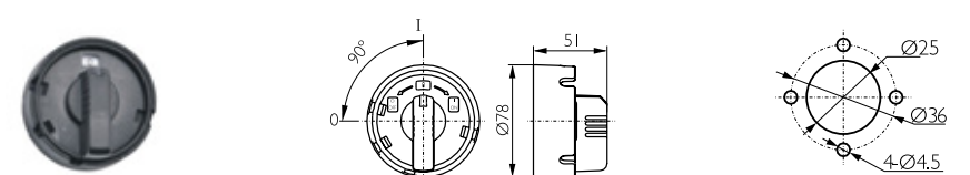
DVACC8003/5PD. OPERATION HANDLE (BLACK) (Ø78mm)
