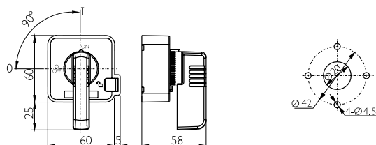
DVACC8029/2BB. SWITCH HANDLE (GREY / BLACK) (60x60mm)
