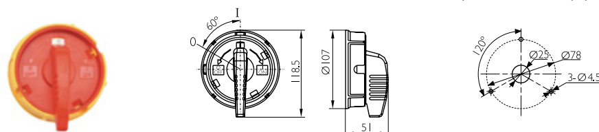
DVACC8003/3DE. EMERGENCY STOP SWITCH HANDLE (RED / YELLOW) (Ø107mm)
