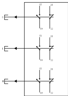
3 Push buttons INO + INC
